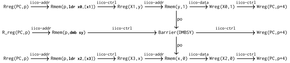
Figure 2.16: Sketch of a completion of reader thread of MP+dmb.sys with implicit events. Nodes and edges include the implicit register or instruction fetch events which are part of the ISA definition (with implicit events corresponding to system register accesses and translation elided for brevity).
