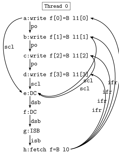
Figure 3.27: Code listing and execution diagram for SM8+sclcachesync-isb.
