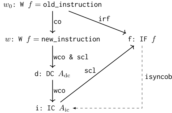
Figure 5.4: General isyncob shape.
