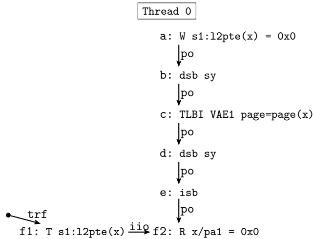
Figure 8.48: Test InvalidateWideBlock
