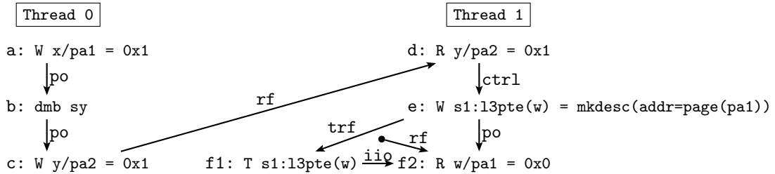
Figure 8.22: Test MP.RT.inv+dmb+ctrl-trfi
