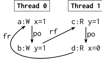
Figure 2.2: MP test execution diagram.
