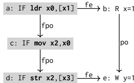
Figure 5.1: An example showing how po is derived from fpo and fe from the implicit fetch events (in grey).
