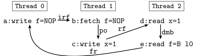
Figure 3.17: Code listing and execution diagram for WRC.F.RR+po+dmb.
