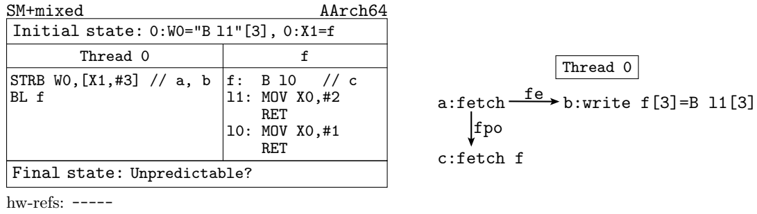
Figure 3.28: Code listing and execution diagram for SM+mixed.
