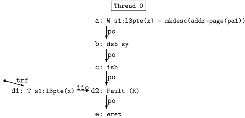
Figure 8.13: Test CoWTf.inv+dsb-isb
