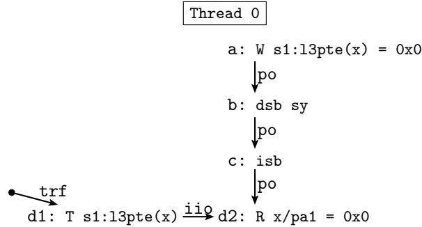
Figure 8.30: Test CoWinvT+dsb-isb
