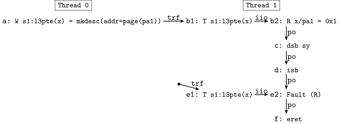
Figure 8.14: Test CoTTf.inv+dsb-isb
