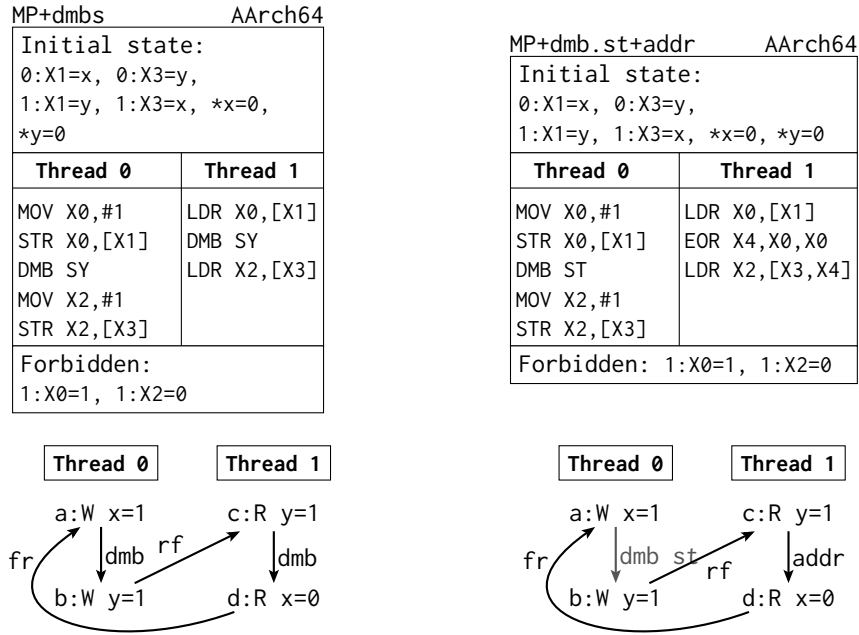
Figure 2.3: Two variants of MP with thread-local ordering. On the left: MP+dmbbs with Arm DMB barrier between instructions. On the right: MP+dmb.st+addr with an address dependency between the reads.
