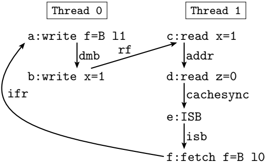
Figure 3.22: Code listing and execution diagram for MP.RRF+dmb+addr-cachesync-isb.
