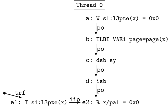
Figure 8.37: Test CoWinvT.EL1+tlbi-dsb-isb
