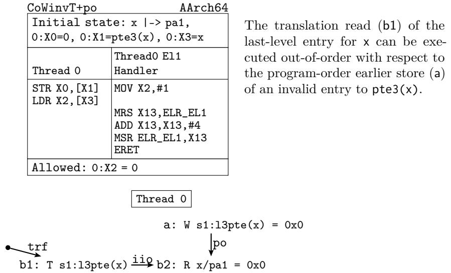
Figure 8.29: Test CoWinvT+po
