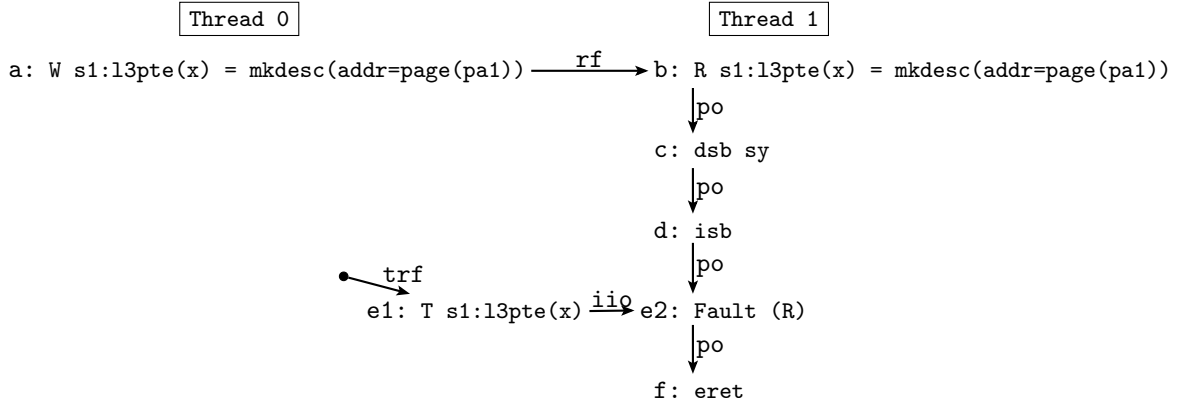
Figure 8.15: Test CoRpteTf.inv+dsb-isb
