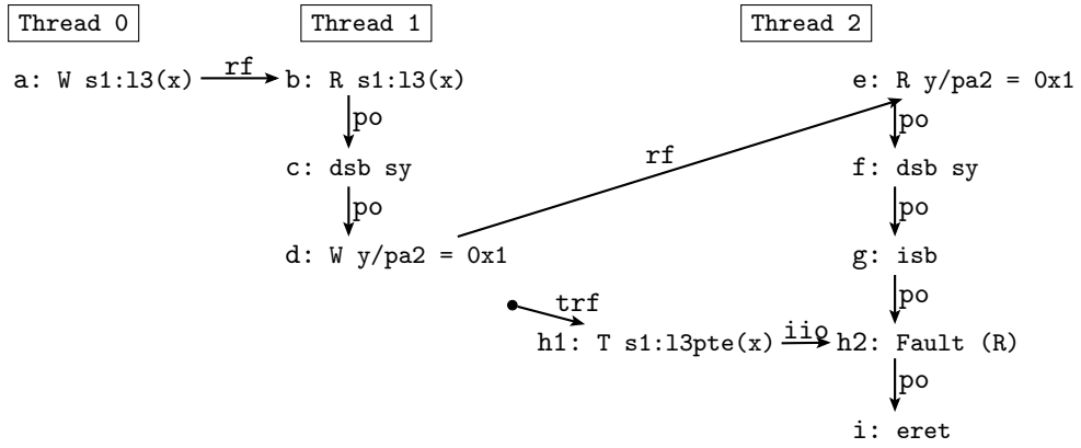
Figure 8.26: Test WRC.RRTf.inv+dmb+dsb-isb
